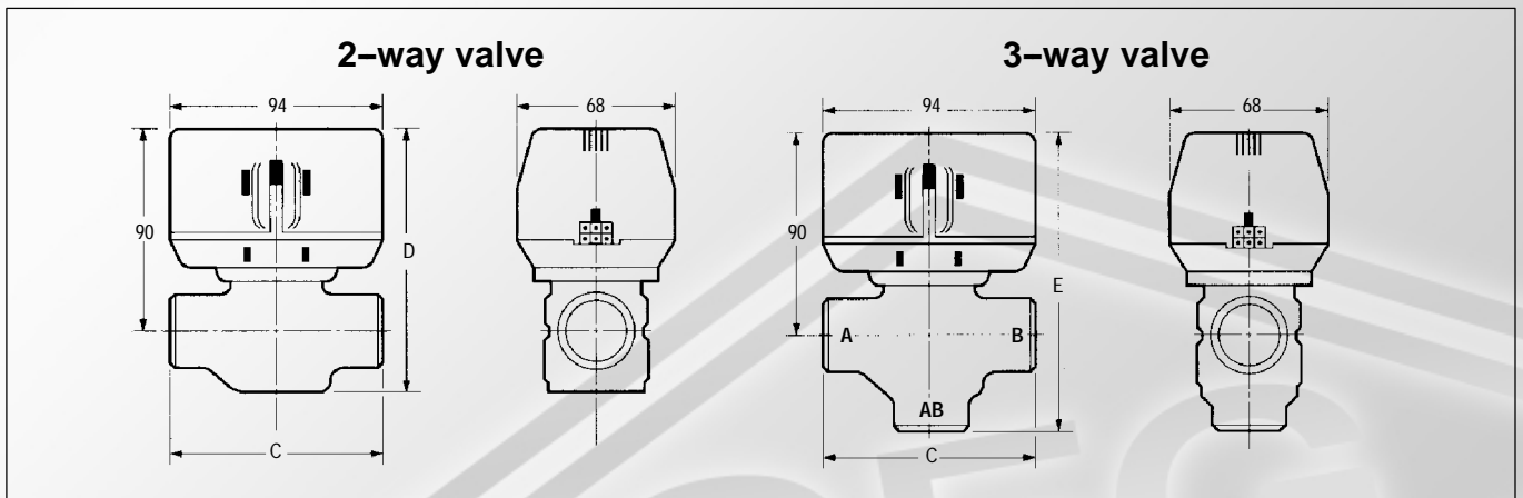
Fig. 10. Valve dimensions
