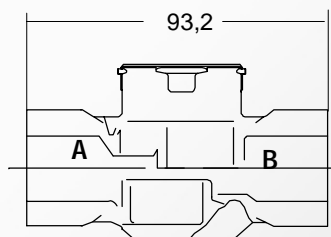
FINISHED DIMENSIONS OF BRONZE BODIES (VC VALVES)
