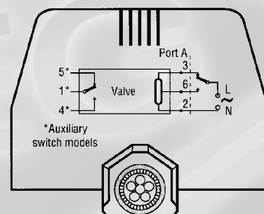
Leadwire cable
