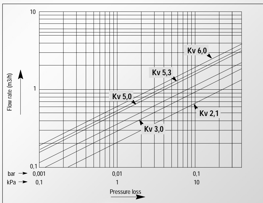
Fig. 8. Valve pressure loss characteristic for 2-way valves
