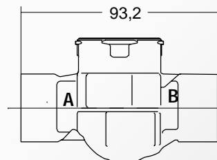
FINISHED DIMENSIONS OF BRONZE BODIES (VC VALVES)
