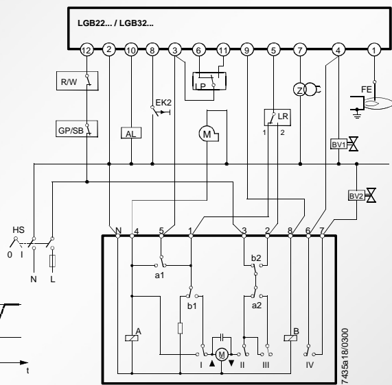
SQN7...424 / two-stage control Two-wire control
