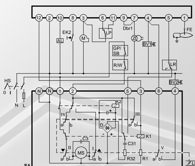
SQN91.140... / two-stage control
