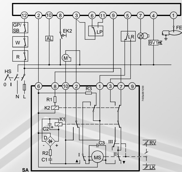
SQN90.220... / two-stage modulating control
